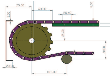
25.4 HASIR BAND DİŞLİ Z.15
