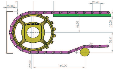
25.4 HASIR BAND DİŞLİ Z.18
